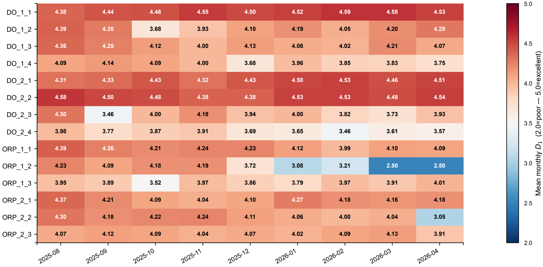
Figure 2. Per-channel monthly D_1 heatmap (v1.1, DO/ORP n=14)
